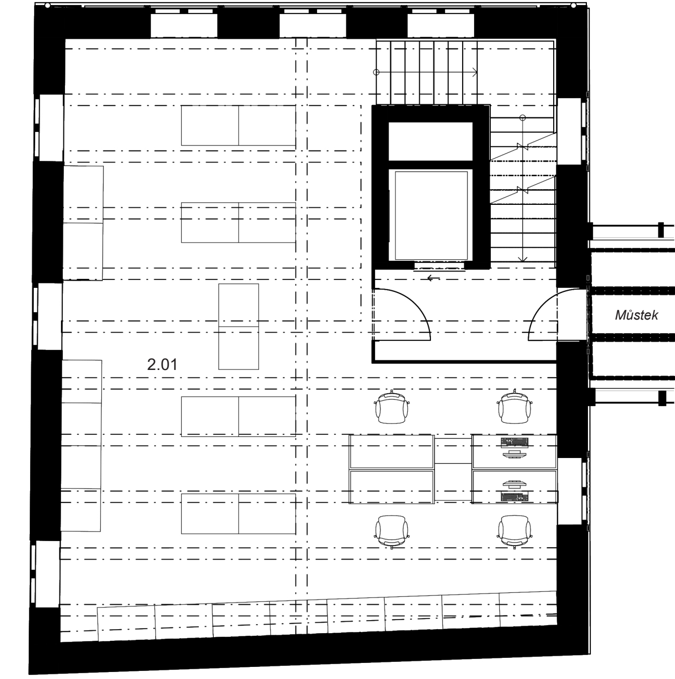
PŮDORYS 2. NP / FLOOR PLAN 2 ND FLOOR
